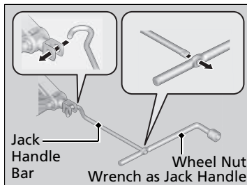
Jacking Point
